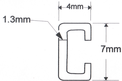
C - SHAPED HOOK
