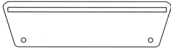
TRAPEZOID SHAPED SLOTTED & DRILLED BROOCH PLATE (WEIGHT 3.5g \pm 0.05g )
